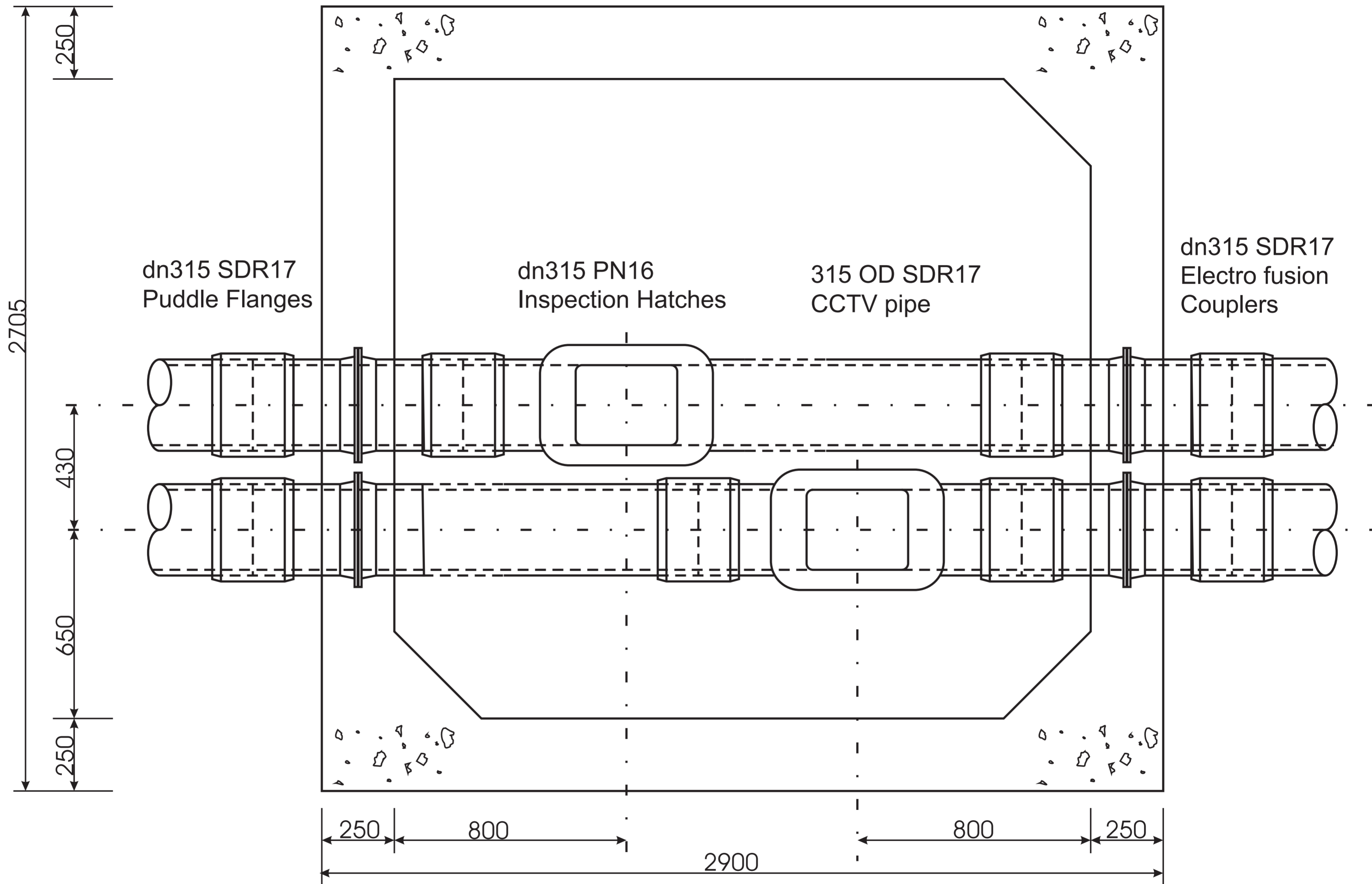
TYPICAL 315 OD SEWER RISING MAIN INSPECTION CHAMBER DESIGN
